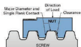
Side Loaded Centralized 'C' Class Nut
