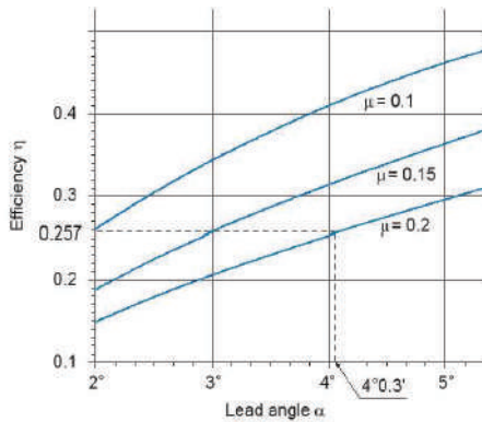
Fig.4 Efficiency
