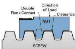
Side Loaded Conventional
