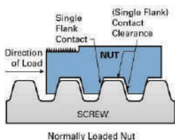
Normally Loaded Nut
