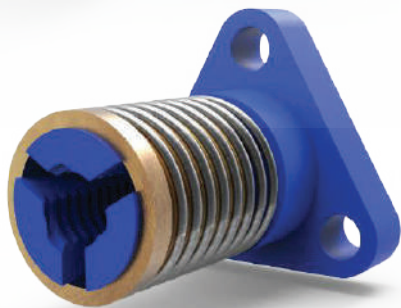
AXIAL LOADED ANTIBACKLASH NUT
